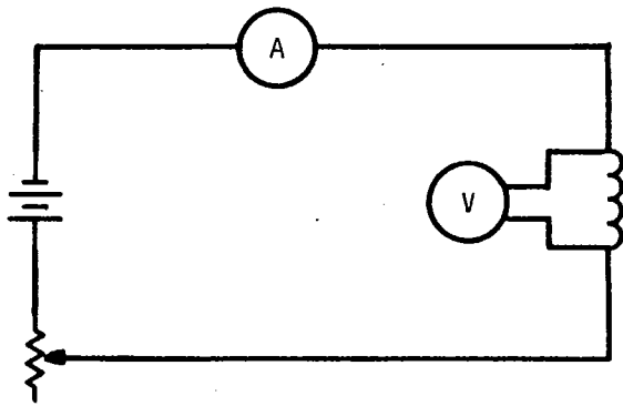
Fig 1 Connections for the Drop-of-Potential Method of Resistance Measurement
