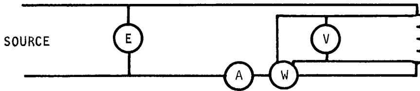
Fig 2 Connections for Impedance Voltage and Impedance Loss Tests
